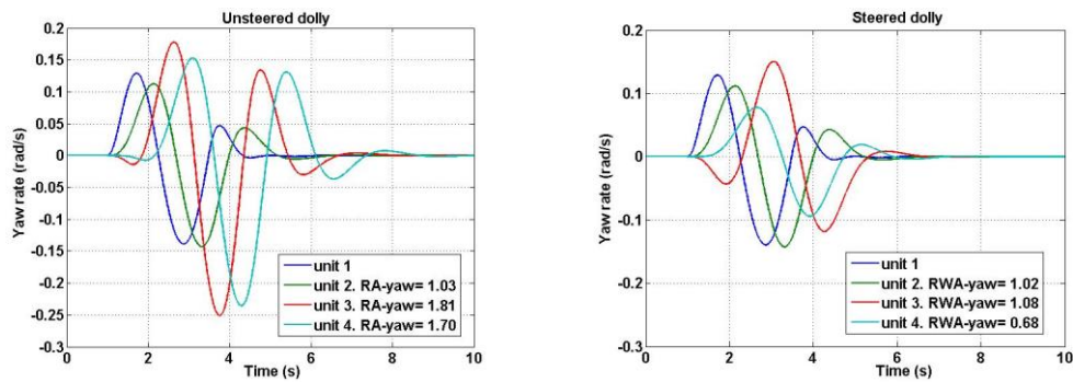
Figure 8 - RWA of yaw rate at velocity of 80 km/h and frequency of 0.4 Hz
